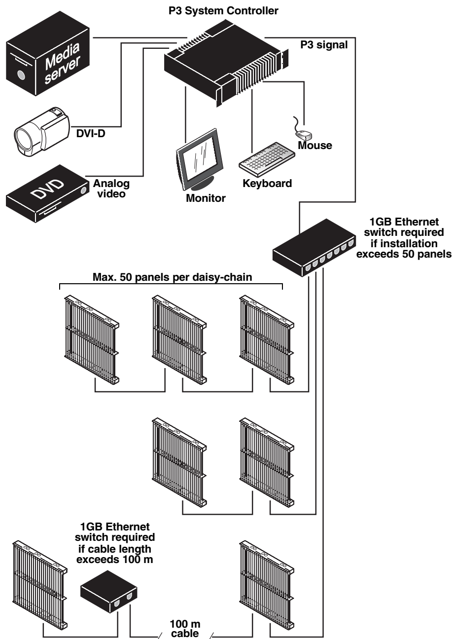
Figure 1: System layout
