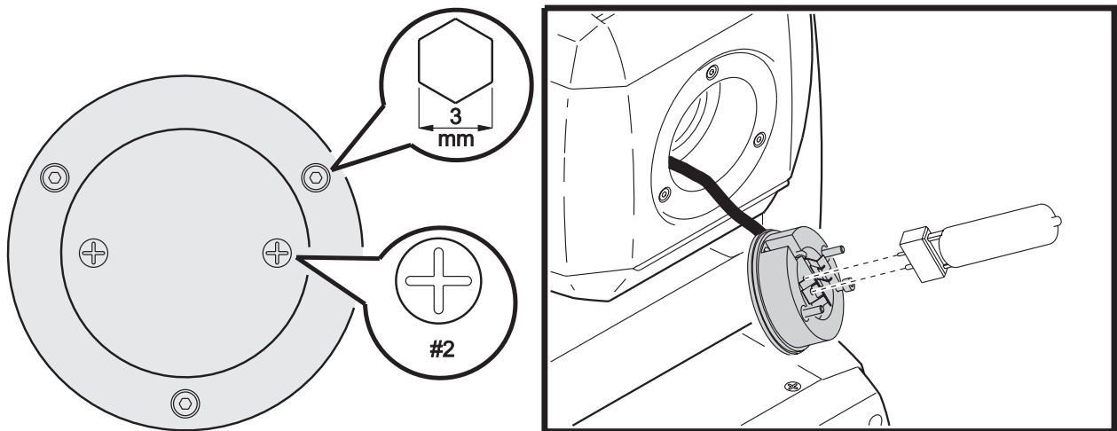
Figure 12: Lamp installation
