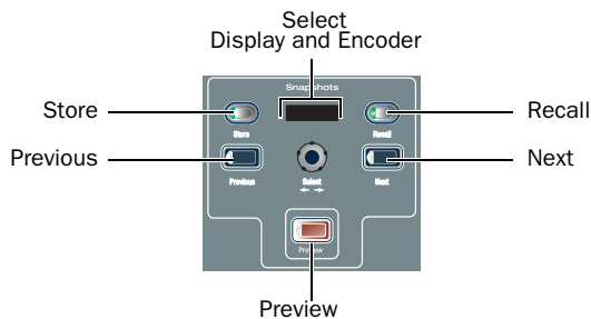
Snapshots section on the console
