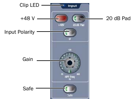
Input controls in the ACS
