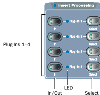
ACS Insert Processing section
