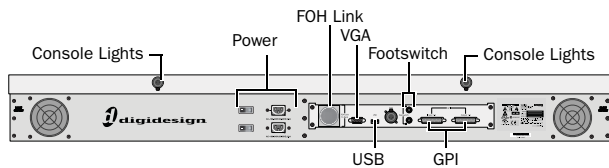
VENUE Profile back panel and connectors
