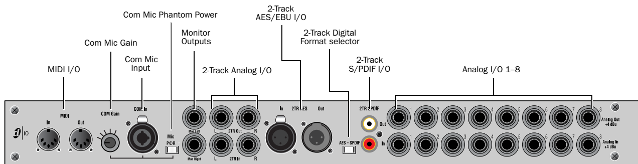
Figure 4. FOH I/O connectors on Mix Rack
