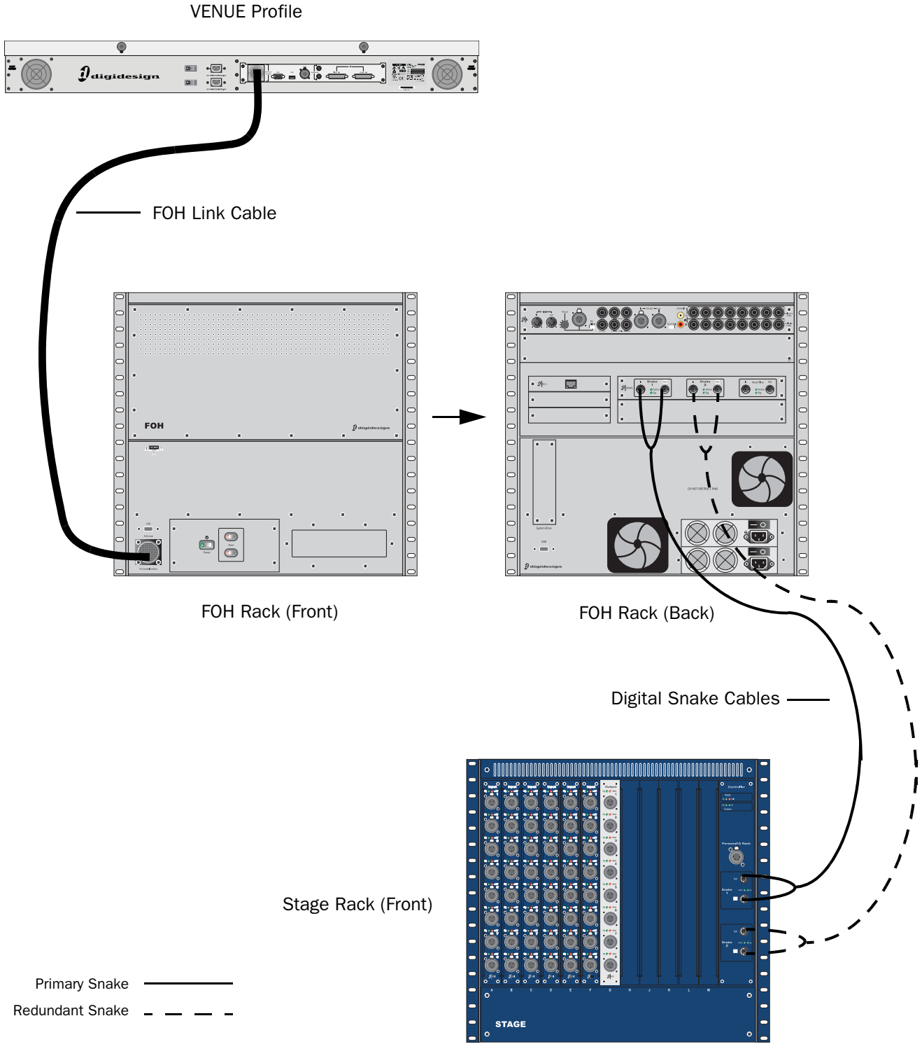
Figure 5. VENUE Profile system component connections
