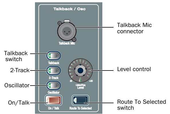
Talkback controls in the Talkback/Osc section
