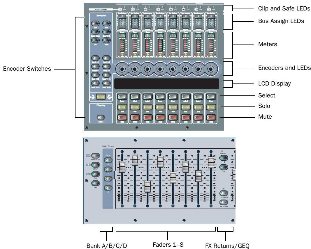
Figure 12. Input controls (Input Channels 1–8 shown)
