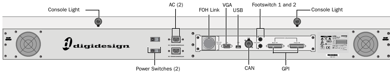
Figure 21. D-Show Profile back panel
