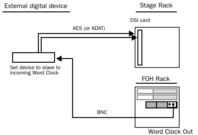
Using word clock from the FOH Rack to clock an external device
