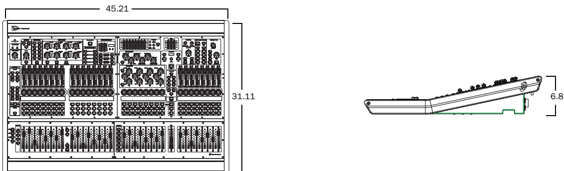
VENUE Profile dimensions
