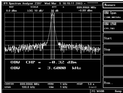
Occupied bandwidth
